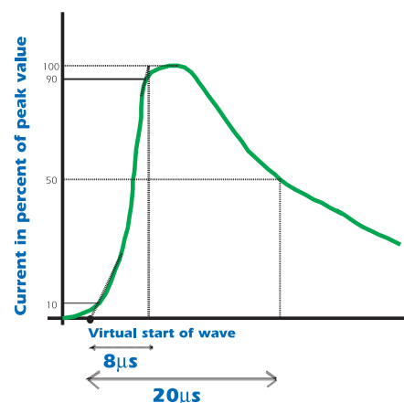
DEFINITION OF THE STANDARD 8/20MS WAVE
