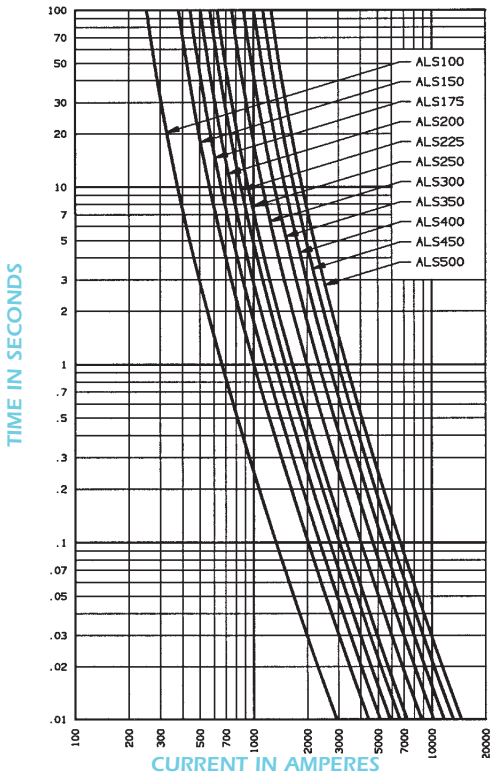
MELTING TIME – CURRENT DATA – ALS100–500
