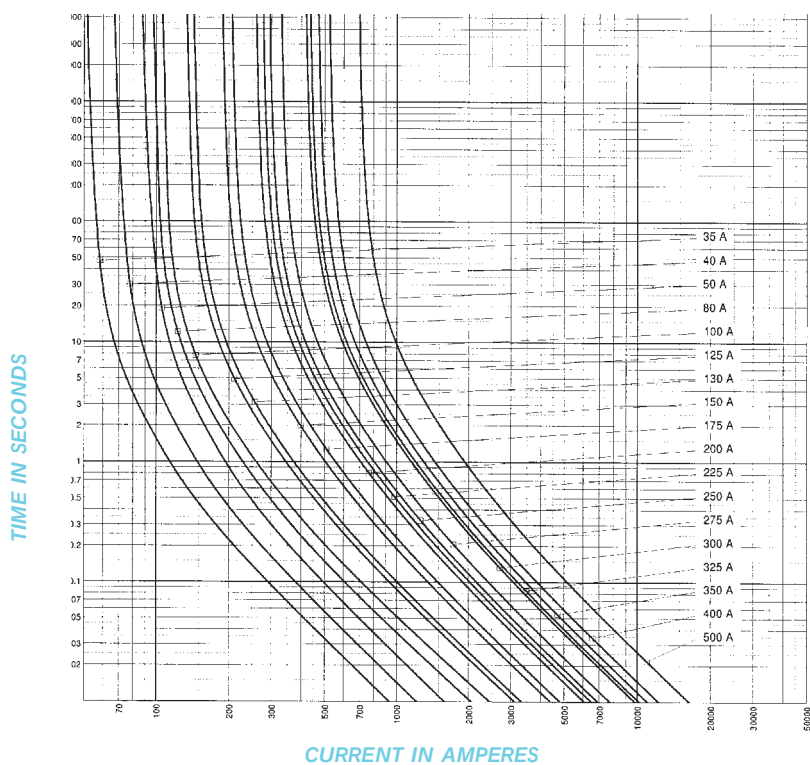
MELTING TIME - CURRENT DATA - CNL35-500
