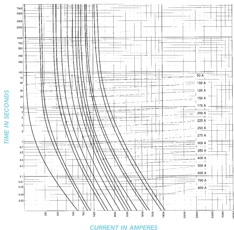
MELTING TIME - CURRENT DATA - CNN10-800
