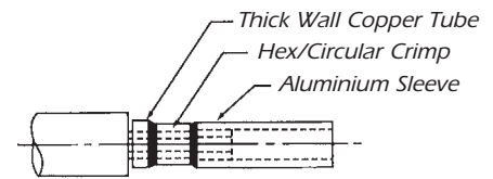
Typical Terminal Assembly Details
